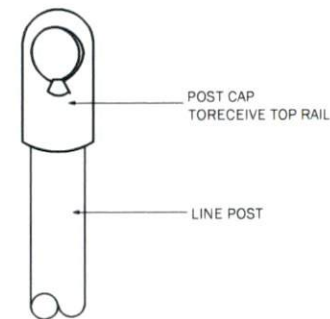
POST CAP DETAIL TYP. N.T.S.
